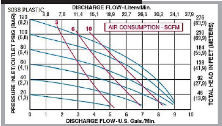
PERFORMANCE CURVE
